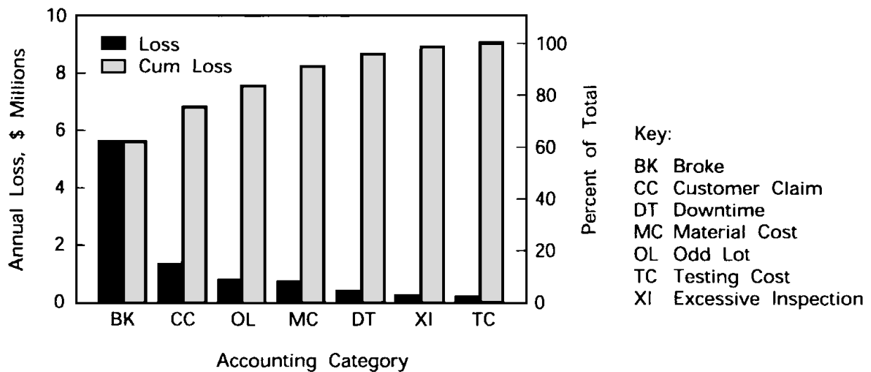
FIGURE 5.8 Pareto analysis: annual loss by category.
