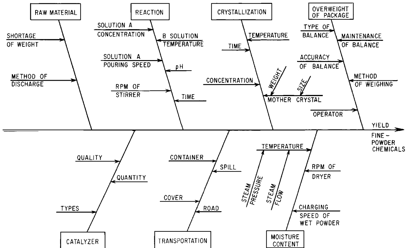
FIGURE 5.14 Ishikawa cause-and-effect diagram.
