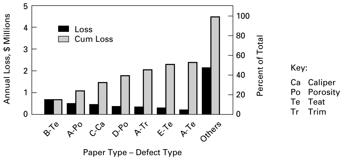
FIGURE 5.10 Pareto analysis: annual loss by defect type.
