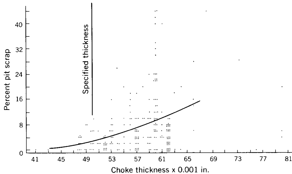
FIGURE 5.18 Test of theories by correlation.
