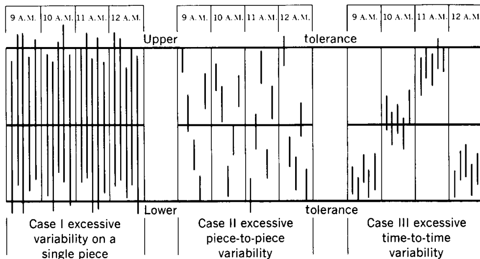
FIGURE 5.15 Multi-Vari chart.
